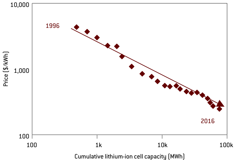
Figure 5: Learning curve of lithium-ion batteries
